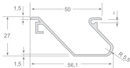
Tirador / Handle Largo/length: 3 mts.
