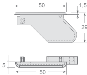
Tapa / Cover Terminal plano Planar end cap
