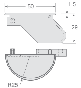
Tapa / Cover Terminal redondo Round end cap
